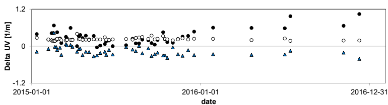
Figure A6. Comparison of UV signal from the sensor ( UV_{Raw} , ●), Lab 2 ( UV_{Lab2 \text{ unfiltered}} , ○), and from Lab 3 ( UV_{Lab3 \text{ filtered}} , ▲) over time.
