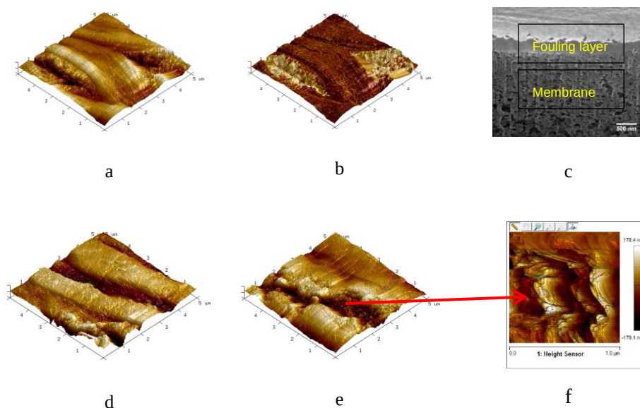
Figure 40 (a) Height sensor and (b) phase images of fouled Aquaflex middle section membrane (scan area: 5×5 μm). (c) SEM image of cross section of Aquaflex middle section membrane showing a ~300 nm fouling layer. (d) Height sensor of fouled Aquaflex membrane (scan area: 5×5 μm). Height sensor of (e) fouled Aquaflex membrane showing micro-cracks (scan area: 5×5 μm) and exposing (f) membrane surface (scan area: 1×1 μm). Figure from Paper II.
