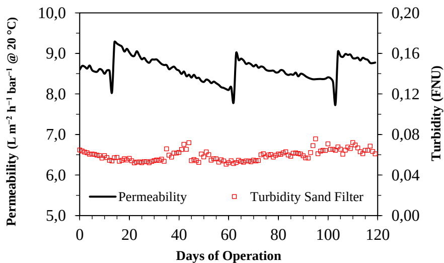
Figure 15 Permeability and turbidity profiles of NF pilot plant before and after CIPs: January 2014 – April 2014. Figure from Paper I.
