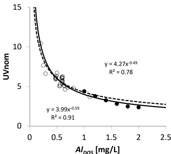
Figure A10. Estimation of normalised UV removal as a function of Al dose based on Equation (4). Black circles (●) are additional high-dose experiments, while white circles (○) are those from the optimization period. Two regression lines including (below) or excluding the additional points are displayed (above).
