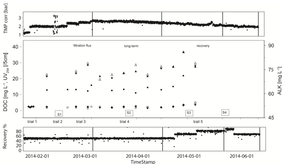
Figure 28 Membrane performance with respect to DOC ( \text{mg L}^{-1} ) (in \bullet and out \circ ), Alkalinity (right scale ( \text{mg L}^{-1} ) ( \text{ALK}_{\text{in}} \Delta , \text{ALK}_{\text{out}} \blacktriangle ), and \text{UV}_{254} ( \text{UV}_{\text{in}} \diamond and \text{UV}_{\text{out}} \blacklozenge ) of the capillary NF container test module for time period January to June 2014 at WTP Görvälnverket, Norrvatten. S1–S4 samples were taken for LC-OCD analysis. Figure from Paper III.
