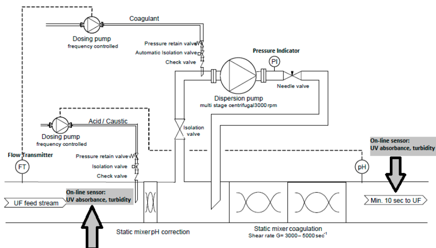
Figure 2. Design for in-line coagulation of full-scale process at Kvarngården WTP.
