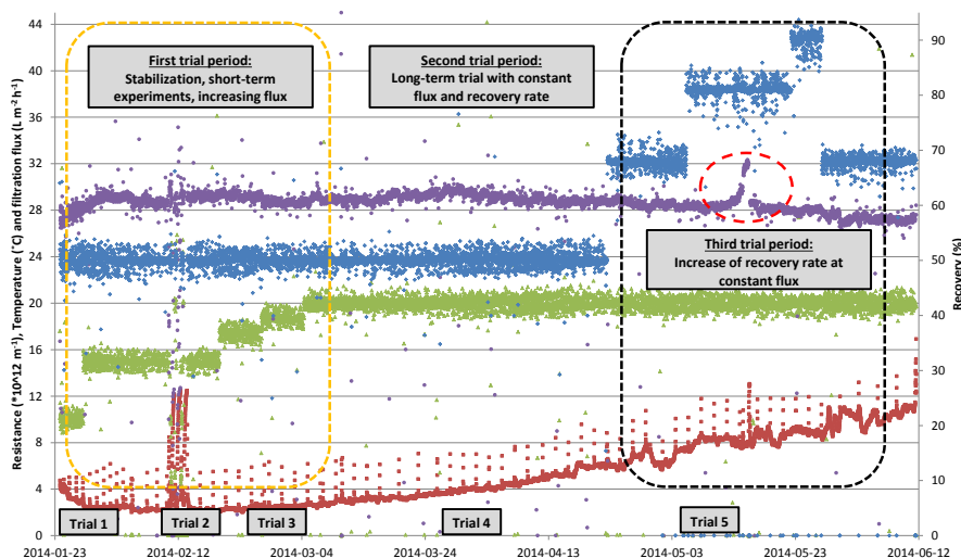
Figure 16 Hydraulic performance of the capillary NF container test module for time period January to June 2014 at G6rv6n WTP, Norrvatten. Periods of increase infiltration flux and increase of recovery rate are marked with orange and black frames respectively. Membrane resistance ( \times 10^{-12} \text{ m}^{-1} ) ( \bullet ), temperature ( ^{\circ}\text{C} ) ( \blacksquare ) and flux rate ( \text{L m}^{-2} \text{ h}^{-1} ) ( \blacktriangle ) on the left y-axis; and recovery rate (%) ( \blacklozenge ) on the right y-axis.
