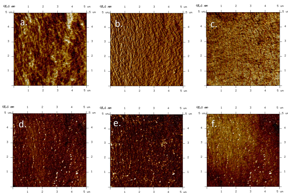
Figure 3. a) Height sensor, b) Peak Force error, c) LogDMT Modulus, d) Adhesion, e) Deformation, and f) Dissipation images of Xiga Center membrane. Scan area: 5×5 μm.
