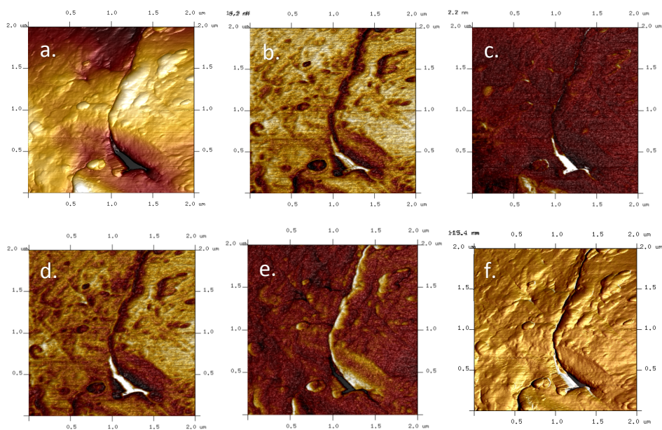
Figure 6. a) Height sensor, b) Adhesion, c) Deformation, d) Dissipation, e) LogDMT Modulus, and f) Peak Force error images of Xiga Left fouled membrane. Scan area: 2×2 μm.
