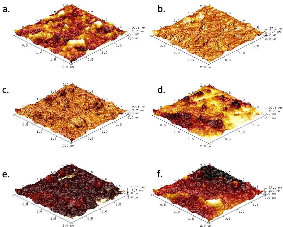
Figure S21. a) Height sensor, b) Peak Force error, c) LogDMT Modulus, d) Adhesion, e) Deformation, and e) Dissipation images of fouled Aquaflex Middle membrane. Scan area: 2 \times 2 \mu\text{m} .
