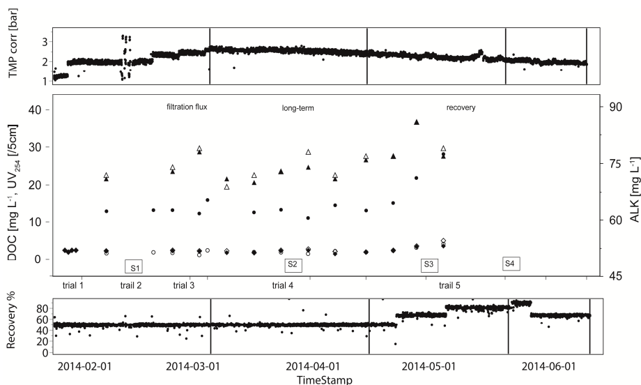
Figure 5. Membrane performance with respect to DOC ( \text{mg} \cdot \text{L}^{-1} ) (in ● and out ○), Alkalinity (right scale ( \text{mg} \cdot \text{L}^{-1} ) ( \text{ALK}_{\text{in}} ▲, \text{ALK}_{\text{out}} △) and \text{UV}_{254} ( \text{UV}_{\text{in}} ◆ and \text{UV}_{\text{out}} ◇) of the capillary NF container test module for time period January to June 2014 at WTP Görvålverket, Norrvatten. S1–S4 and bars as in Figure 3.
