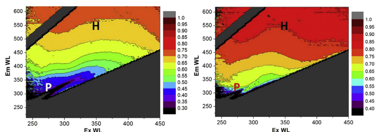
Fig. 3. Fraction of removed fluorescent dissolved organic matter for coagulation (left) and NF (right) treatments. Dark red colors indicate strong removal ( >75\% ) while blue–purple colors indicate less removal ( <40\% ). The excitation/emission wavelength pairs chosen to represent humic-like (Ex = 350 nm, Em = 550 nm, marked “H” in the EEMs) and protein-like (Ex = 276 nm, Em = 320 nm, marked “P” in the EEMs). (For interpretation of the references to color in this figure legend, the reader is referred to the web version of this article.)
