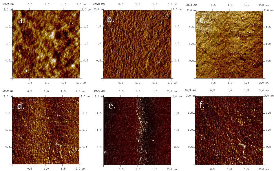
Figure 4. a) Height sensor, b) Peak Force error, c) LogDMT Modulus, d) Adhesion, e) Deformation, and f) Dissipation images of Aquaflex bottom membrane. Scan area: 2×2 μm.
