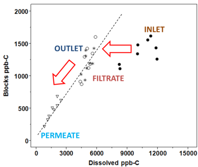
Figure 27 Linear regression of concentrations of different organic matters as a function of DOC concentration in different process streams; Building Blocks vs. DOC. Raw water from Lake Mälaren (●), rapid sand filter filtrate (○), NF permeate (▽), and drinking water from existing treatment process at Görvåln WTP (*). Figure from Paper I.
