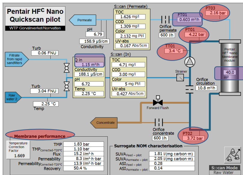
Figure 3 SCADA for NF QuickScan pilot at Görvål WTP, graphical interface & process flow schematic.
