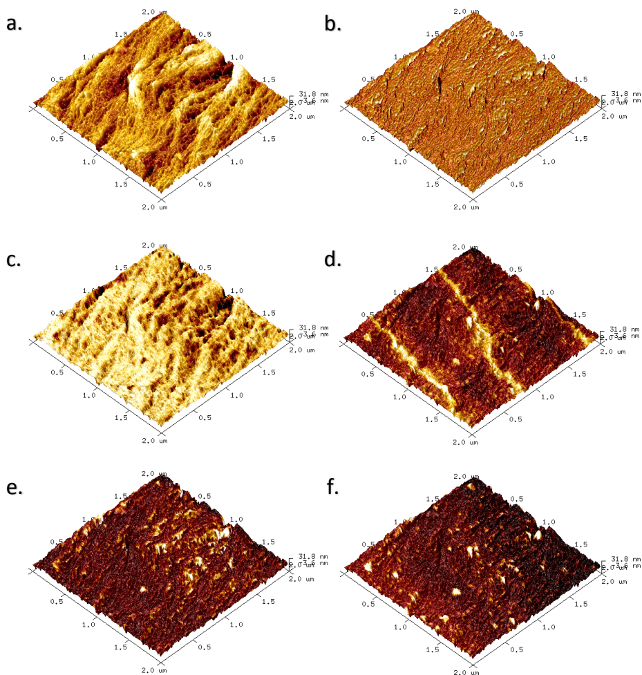
Figure 1. a) Height sensor, b) Peak Force error, c) LogDMT Modulus, d) Adhesion, e) Deformation, and f) Dissipation images of Aquaflex virgin membrane. Scan area: 2×2 μm.
