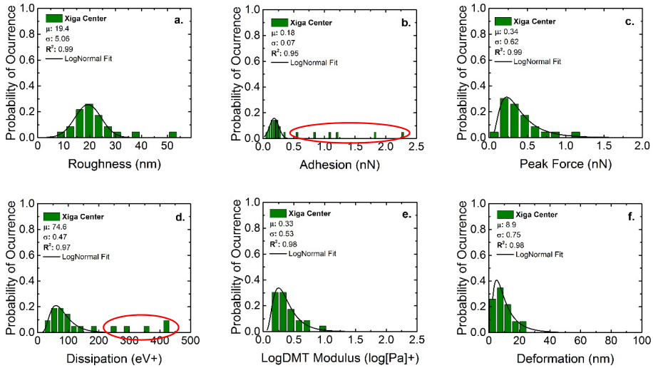
Figure S10. Probability density functions describing a) roughness, b) adhesion, c) Peak Force error, d) dissipation, e) LogDMT Modulus and f) deformation of Xiga center membrane
