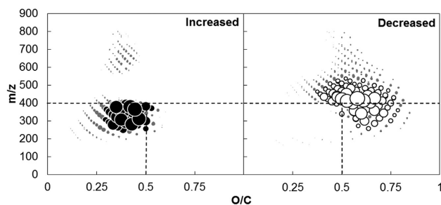
Fig. 5. CHO components that increased (left) and decreased (right) during the pilot scale nanofiltration of, with chemical coagulation, treated water. White and black bubbles demonstrate significant changes in relative abundance while gray bubbles show non significant changes. Bubble size represents the magnitude of the change in relative abundance (maximum 52 percentage point's decrease and 24 percentage point's increase).
