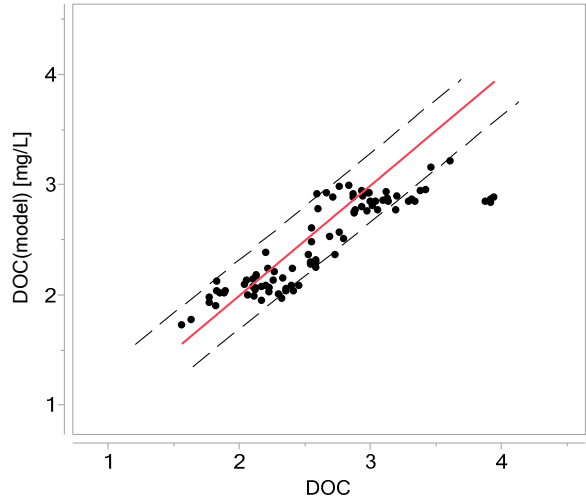
Figure A3. Measured DOC (mg L -1 ) against predicted DOC (DOC (model) = a + b * UV Lab3 filt ). The close linear relationship is proof of extremely stable SUVA over time.
