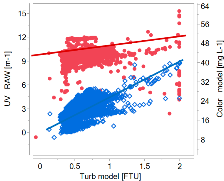
Figure A8. Estimation of effects of sensor-modelled turbidity (FTU) on sensor-modelled colour ( \diamond ), and sensor-measured UV ( \bullet ). UV = 9.30 + 0.523 \cdot Turb_{model} . Per one unit of modelled turbidity, approximately half a unit of UV is added, which is in accordance with unpublished stream data from the Fyris River (Uppsala, Sweden). At turbidity of 2, an additional UV signal of 1 is captured that is not related to the DOC. The offset 9.3 is extremely close to the average raw water UV. Regarding the colour, this effect is more pronounced, such that a turbidity of 2 could give rise to additional colour of 36 \text{ mg L}^{-1} , therefore dominating the signal. Color = 11.6 + 18.4 \cdot Turb_{model} .
