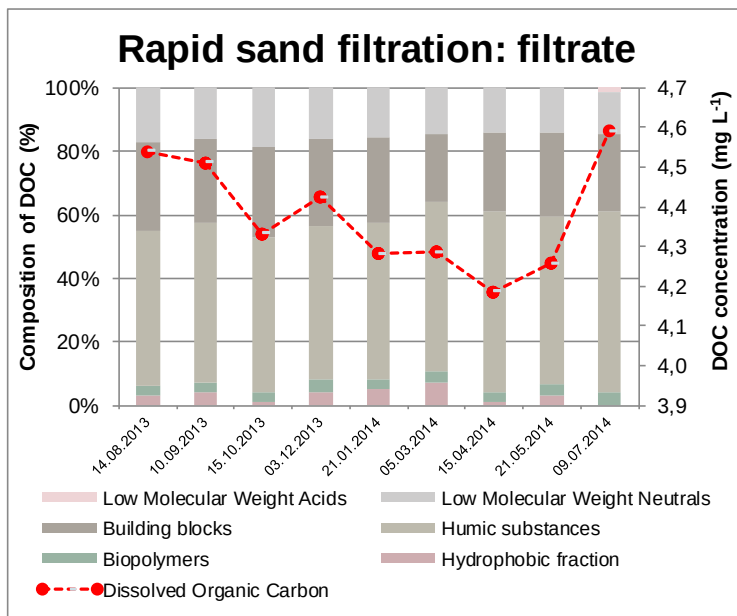
Figure 21 DOC fractionation of filtrate from full-scale rapid sand filtration (RSF) at Görvåln WTP (feed water to NF-pilot plant).
