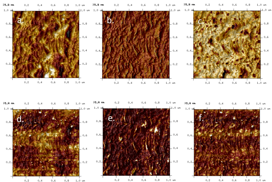
Figure S8. a) Height sensor, b) Peak Force error, c) LogDMT Modulus, d) Adhesion, e) Deformation, and f) Dissipation images of Xiga virgin membrane. Scan area: 1×1 μm.
