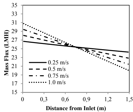
Figure 6: water flux distribution along module length at different cross-flow velocities
