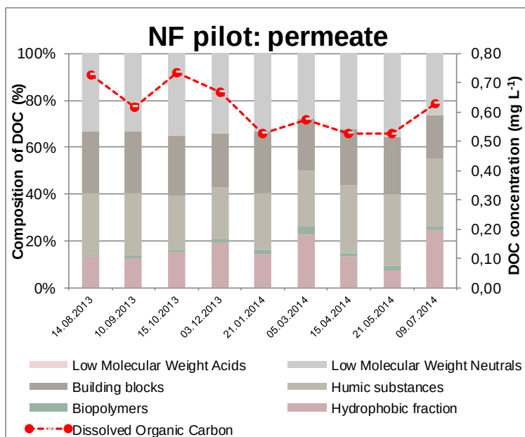
Figure 22 DOC fractionation of permeate from NF pilot plant at Görvåln WTP (feed water: RSF filtrate from full-scale treatment).
