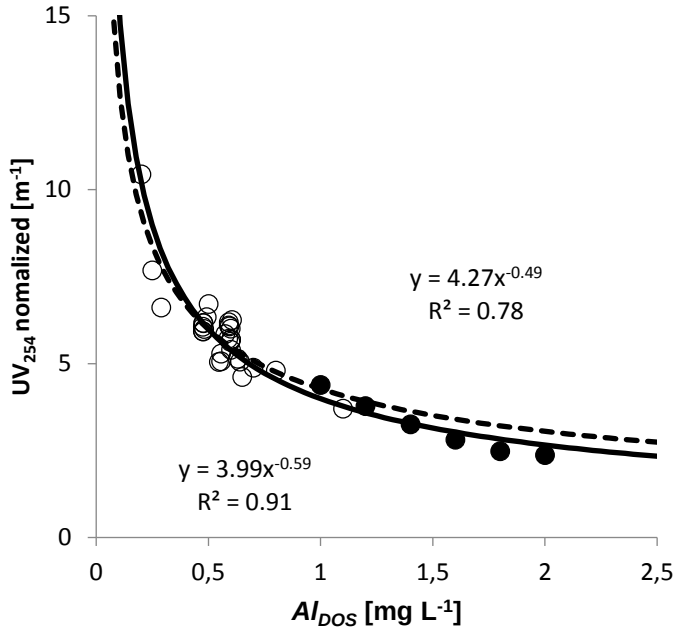
Figure 34 Estimation of normalized UV 254 removal as a function of Al dose based on Eq.(4). Black circles (●) are additional high-dose experiments, while white circles (O) are derived from the optimization period during long-term UF pilot trials at Kvarngården WTP. Two regression lines are depicted including (below) or excluding (above) the additional data points for high-dose test runs. Figure from supplementary information to Paper V.
